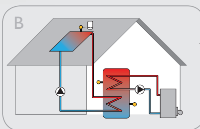
Solar collector & solar tank, gas booster
