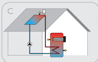
Solar collector & solar tank, electric booster (incl. auxiliary relay)
