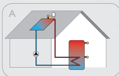
3 sensors, solar collector & solar tank
