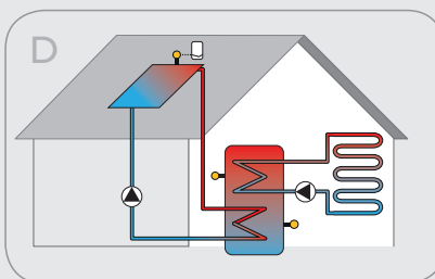
Solar collector & solar tank, hydronic floor system
